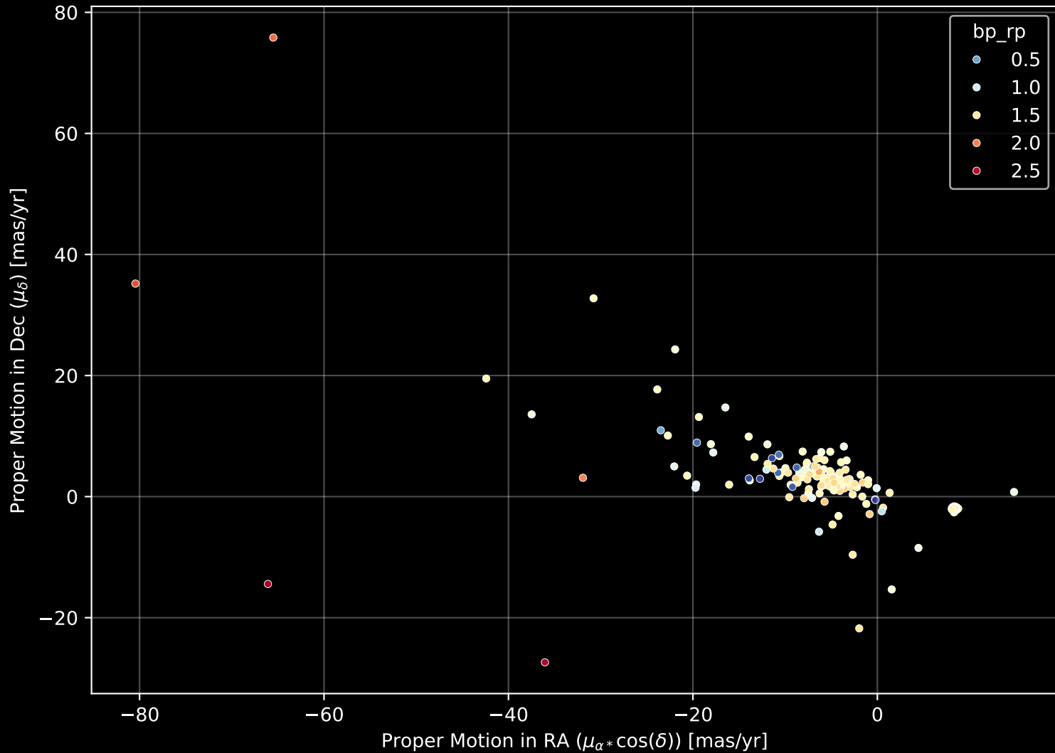
APOGEE DR17 Field: [N3201] Proper Motion Diagram (n= 249)
