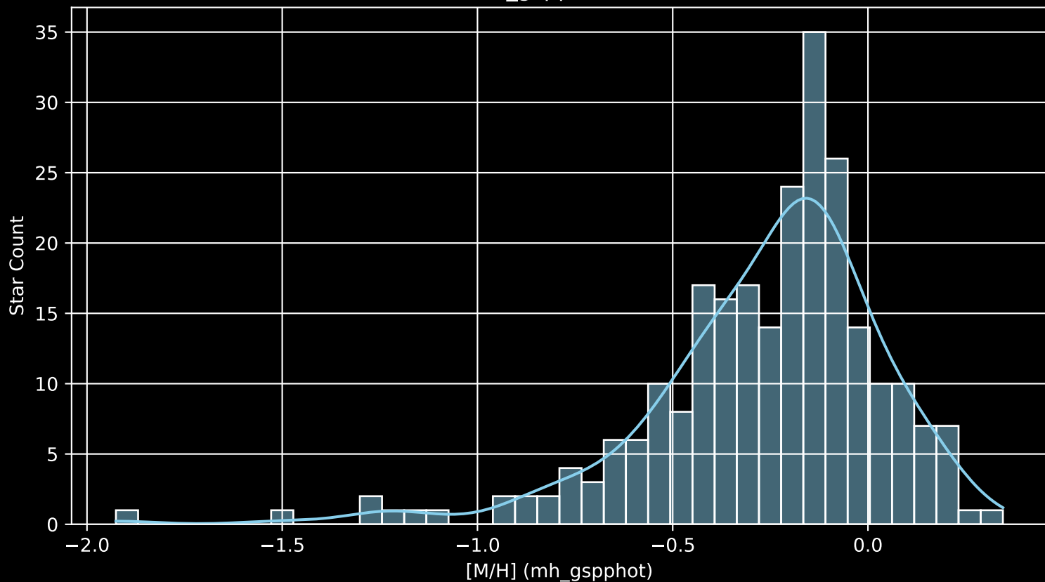
APOGEE DR17 Field: [N3201 [M/H] (mh_gspphot) (n= 249)
