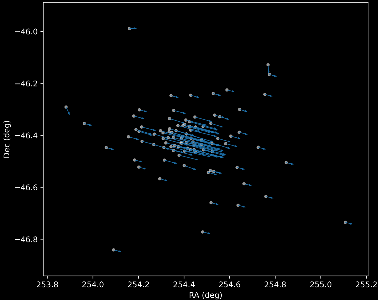
APOGEE DR17 Cluster 0 Proper Motion Vectors (n=93)
