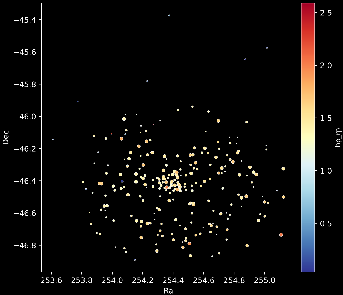
APOGEE DR17 Field: [N3201] Stars: 249
