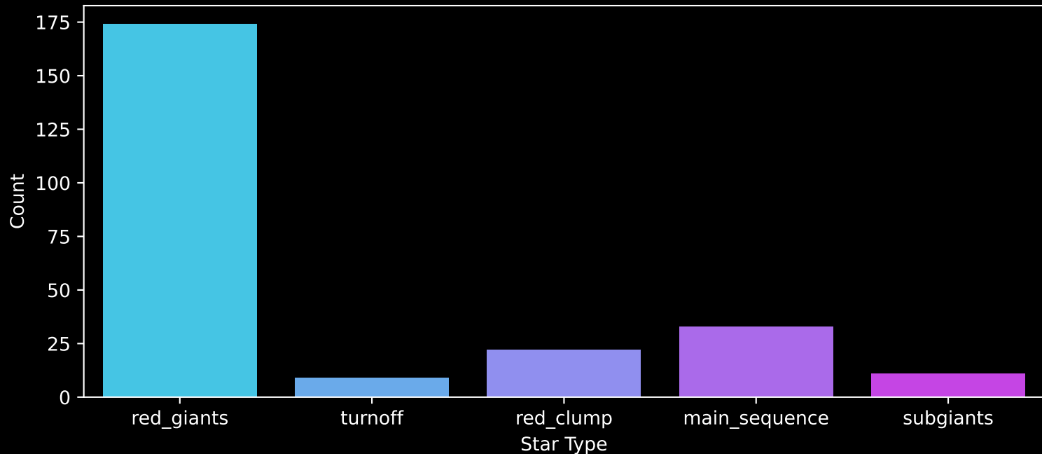
APOGEE DR17 Field: [N3201] Count plot of Star Type
