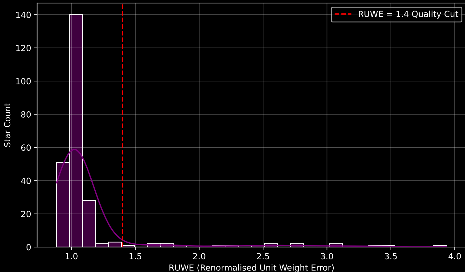
GAPOGEE DR17 Field [N3201] RUWE Distribution (n= 242)
