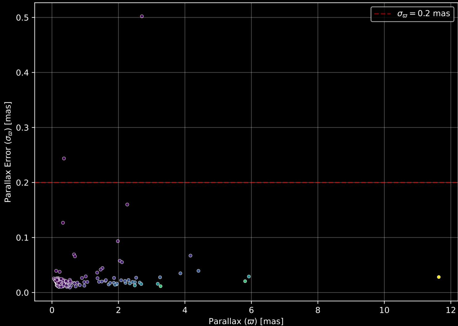
APOGEE DR17 Field: [N3201] Parallax Quality (n= 249)
